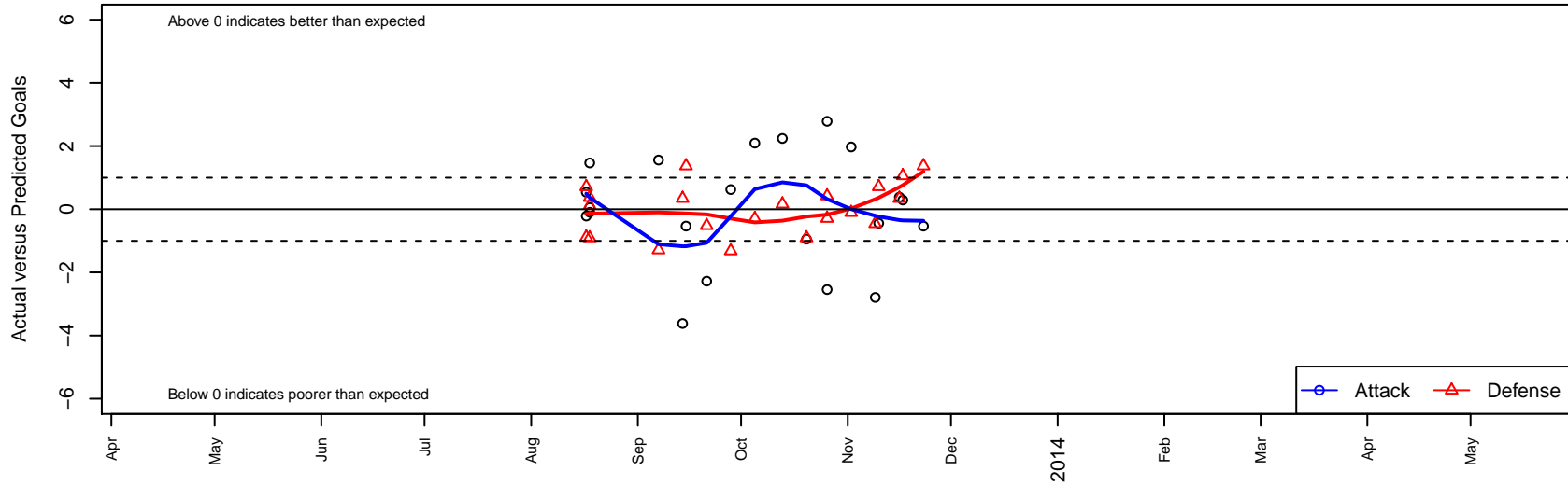
LA Galaxy Academy South B01 Dots are actual minus expected GF (blue circles) and GA (red triangles). Blue line is smoothed change in attack strength. Red is smoothed change in defense strength.
